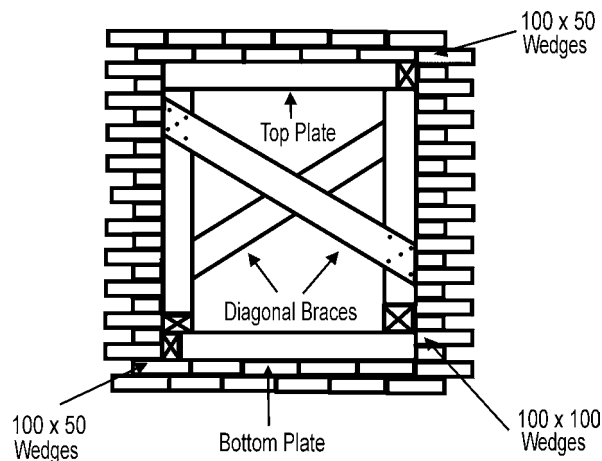
Figure 15:18 Diagonal bracing
