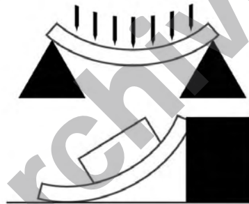
Figure 14:12 Force type bending (load)
