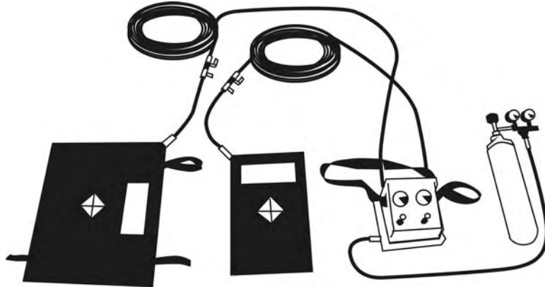
Figure 11:11 Airbag system
