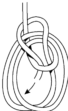
Figure 5:22 Portuguese Bowline
