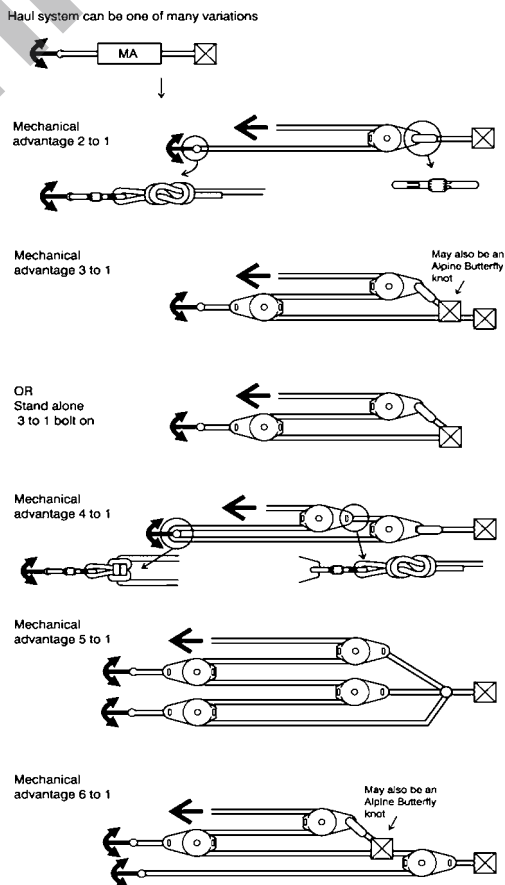
Figure 9:8 Lightweight pulley systems
