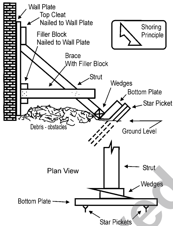
Figure 15:9 Split brace shore
