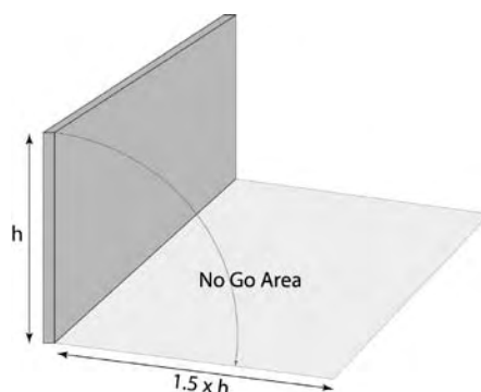
Figure 14:15 Collapse zone
